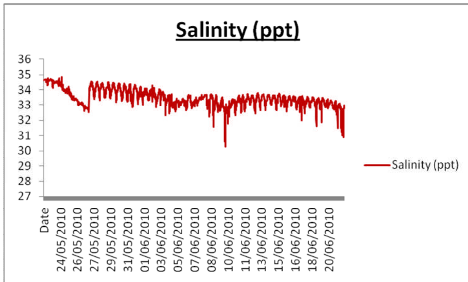
Graph showing the salinity readings provided by the data buoy
