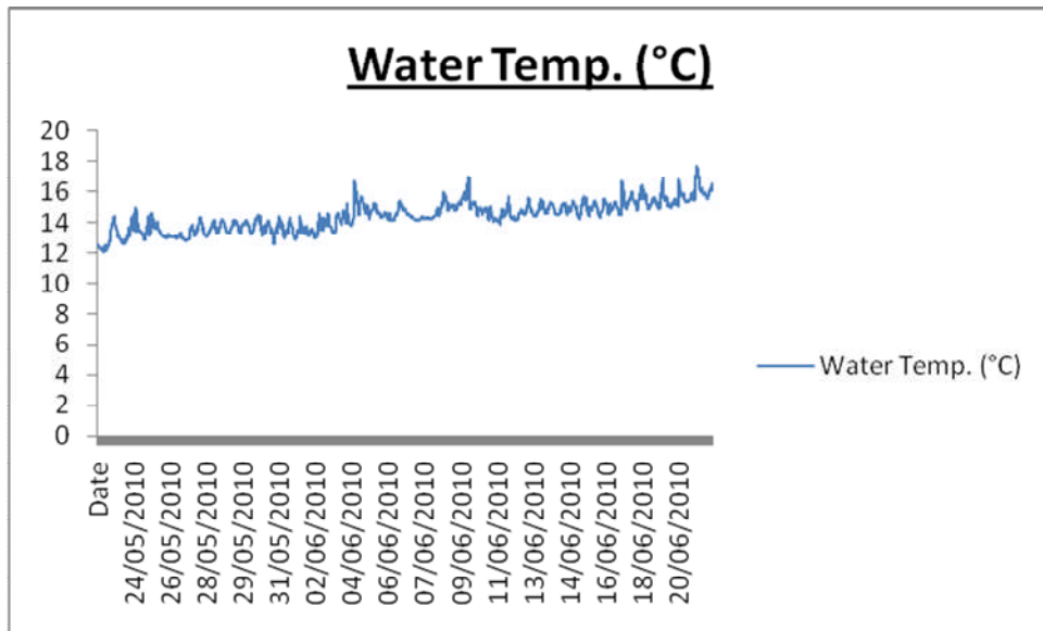
Graph showing the water temperature readings provided by the data buoy
