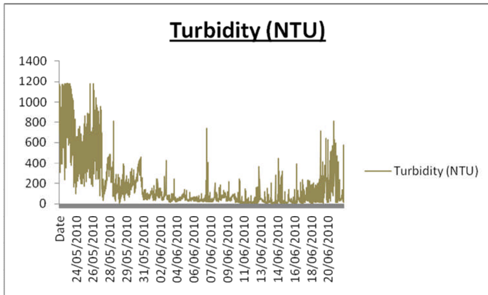
Graph showing the turbidity readings provided by the data buoy
