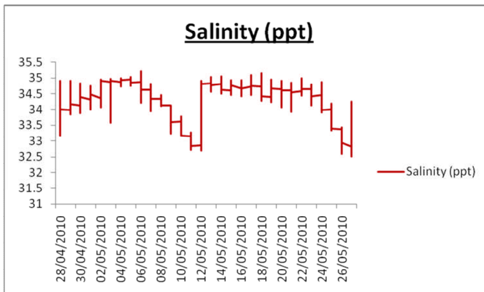
Graph showing the salinity levels within the Falmouth Estuary April-May 2010
