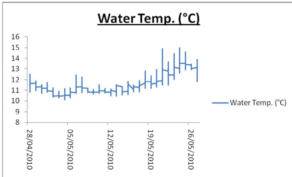
Graph showing the water temperature of the Falmouth Estuary April-May 2010
