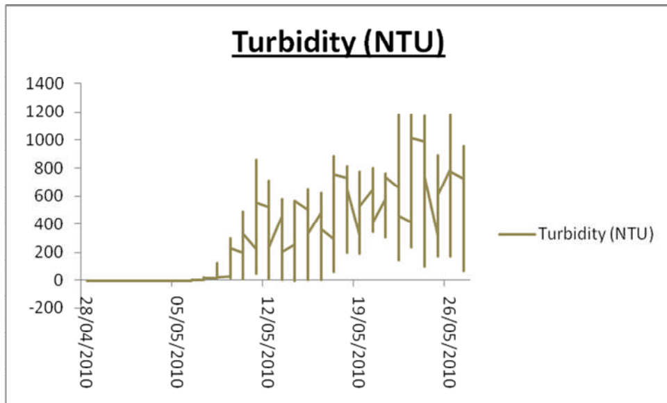
Graph showing the turbidity levels within Falmouth Estuary April-May 2010
