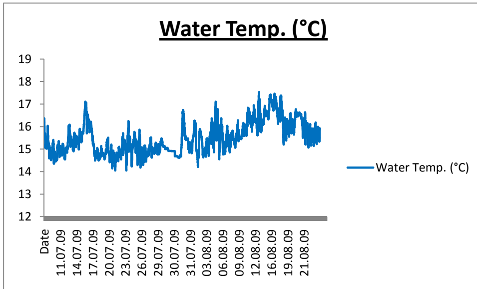
Graph showing the water temperature readings provided by the SANY buoy
